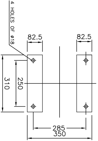
PLAN OF PUMP FEET
